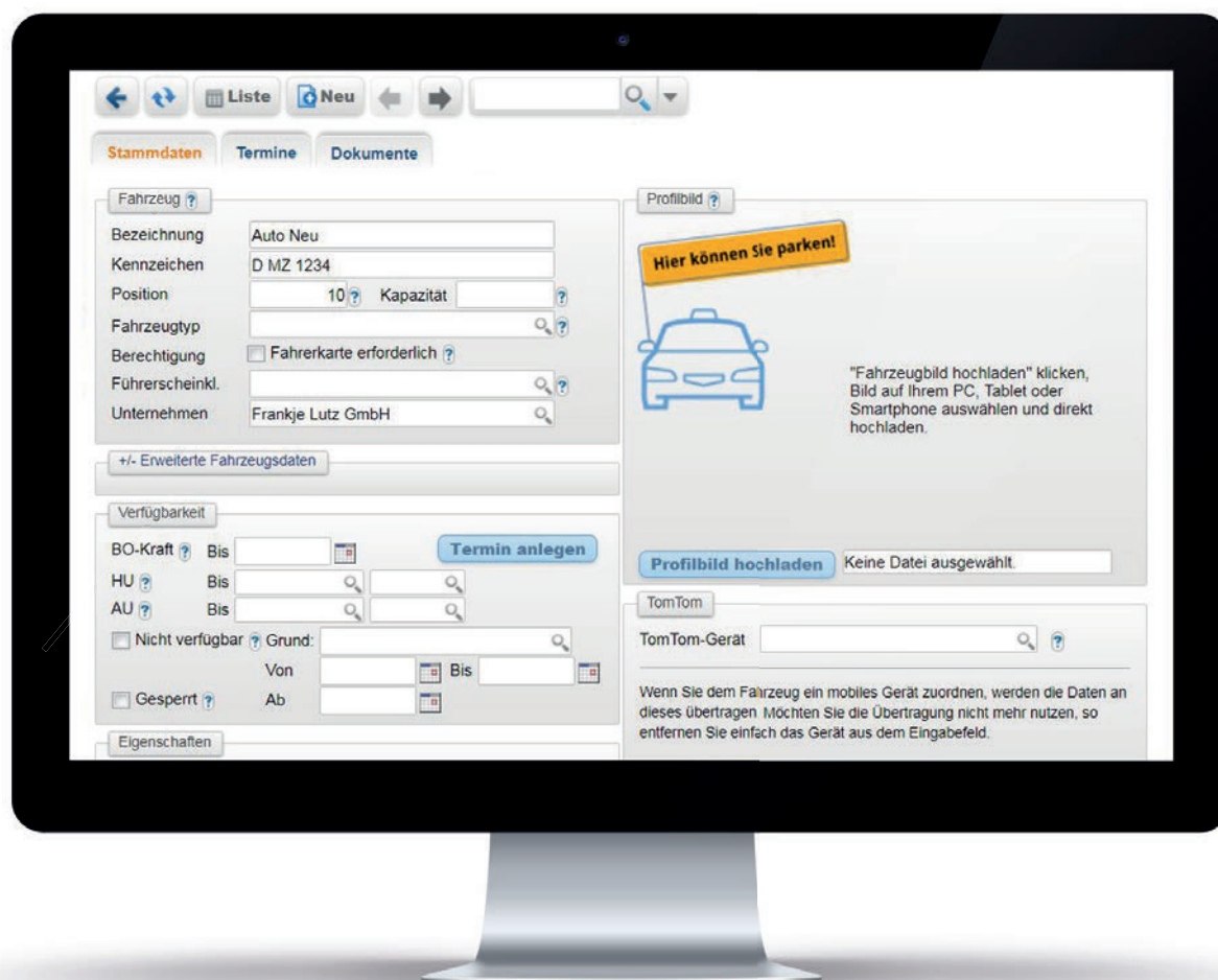
Fuhrparkmanagement
